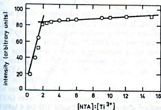
Fig. 4. Establishment of the ratio [Ti(III)] to [NTA] at pH 9.1, 0.01 M- TiCl_3 , by the mole ratio method, the absorption maximum at \tilde{\nu} = 16700\text{ cm}^{-1} .
