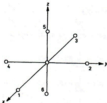
Fig. 10. Coordinate axes and numbering for the tetragonal d^1 system.
