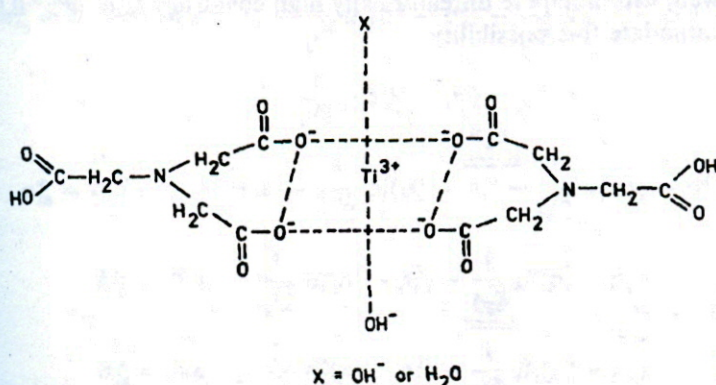
Fig. 8. Model of Ti(III) coordination in \text{trans-}[\text{Ti}(\text{NTA})_2\text{X}_2] .
