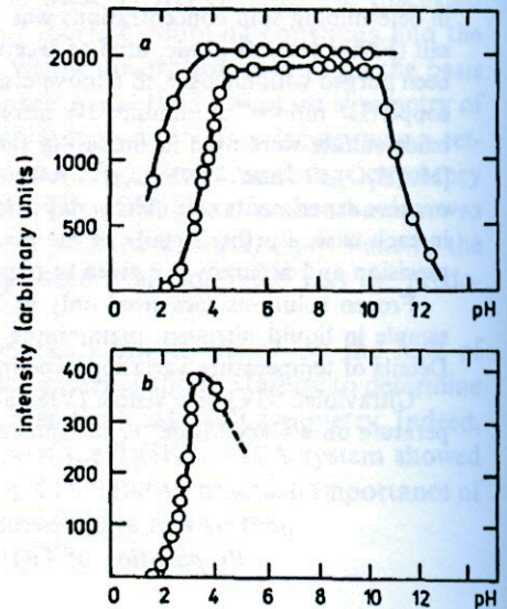
Fig. 2. a) The pH dependence of proposed Ti(NTA) 2 complex ion. Upper curve: absorbance at \nu = 14000\text{ cm}^{-1} , lower curve: ESR signal intensity. 0.02 M-TiCl 3 , [Ti 3+ ]:[NTA] = 1:20.
